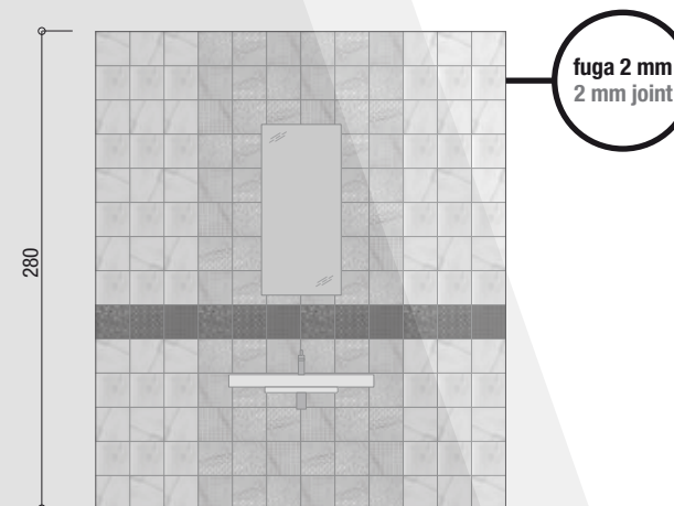
Wall A
