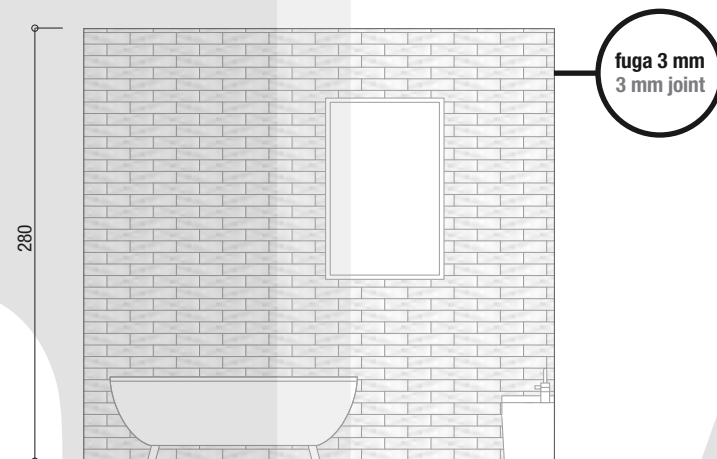
Wall A
